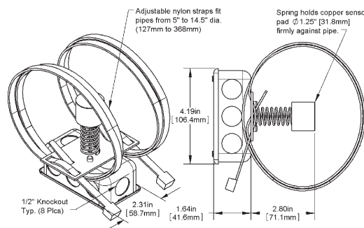
Spring-Loaded Strap J-Box
