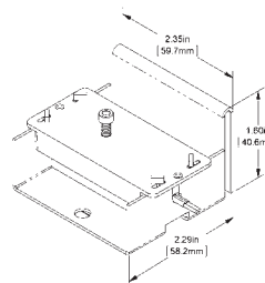
Water Leak Detector with Remote Sensor
