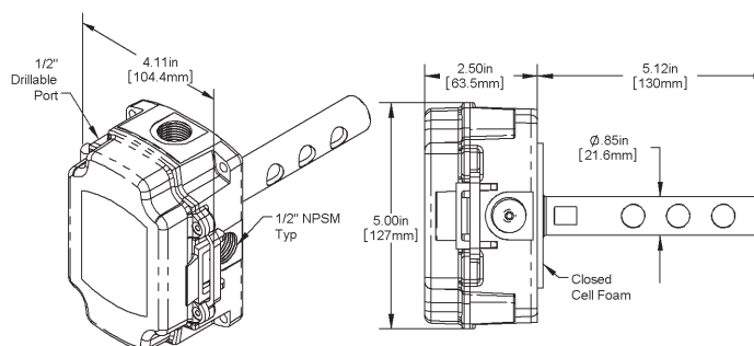
CO 2 Duct Sensor in the BAPI-Box Enclosure
