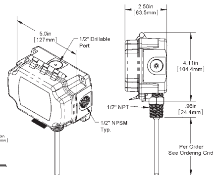
BAPI-Box (BBO) Model in an "Outside Mount" Configuration
