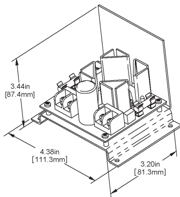
VC3000B Voltage Converter (shown with optional backplate)
