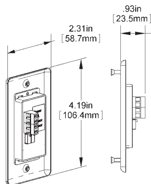
-XOR Model (shown with optional Terminal Block)
