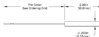
Remote Sensor Probe & Wires
