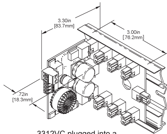
3312VC plugged into a BP4 Backplane
