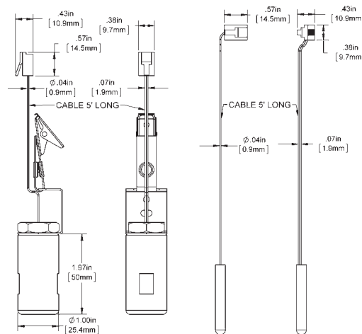
External Hanging Thermobuffer Sensor
