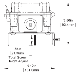
Water Leak Detector with Attached Sensor
