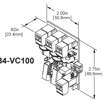
TB4-VC100 Module in an accessory Snaptrack
