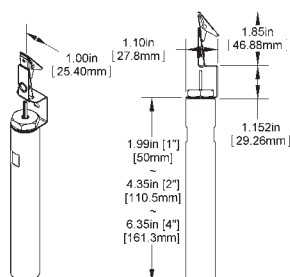
Hanging Bracket
