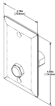
Vivarium Wall Plate Unit
