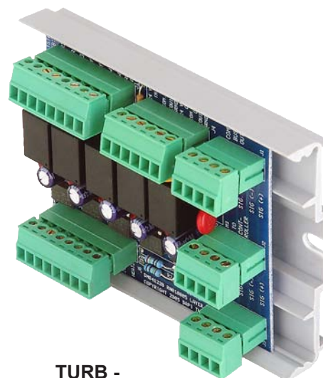
TURB - Terminal Unit Relay Board mounted in the optional 2.75" snaptrack
