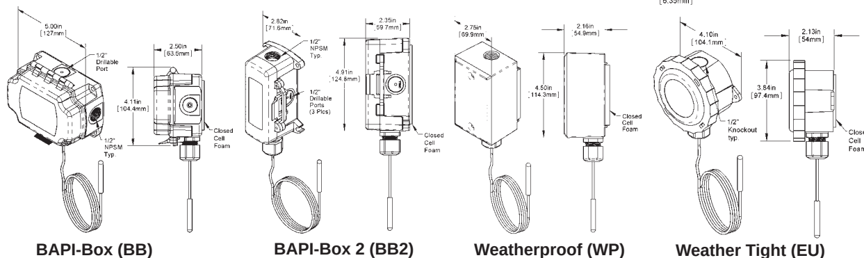
Remote Sensor Probe & Wires
