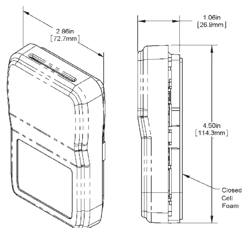
CO 2 Sensor in the BAPI-Stat 4 Enclosure
