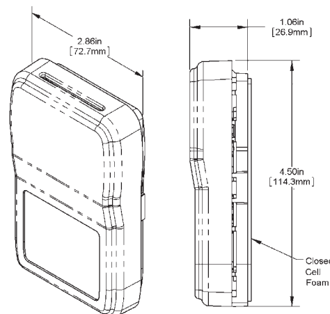
"24/7" CO 2 Sensor in the BAPI-Stat 4 Enclosure
